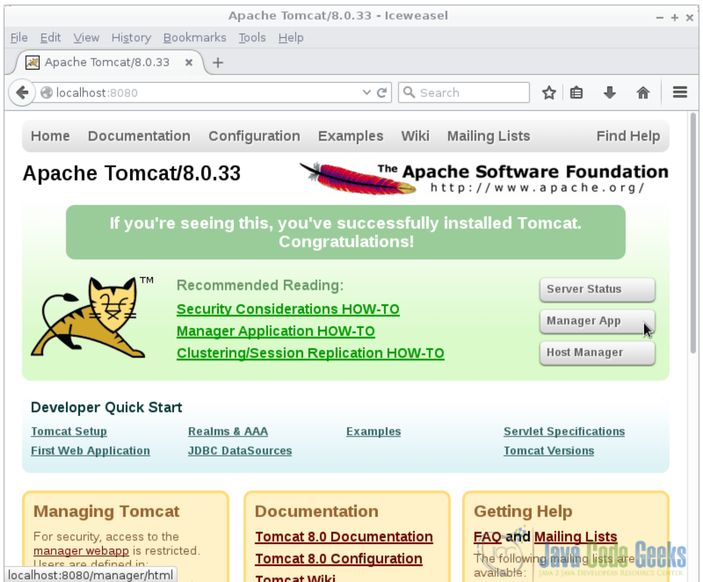
Figure 1.6: Tomcat Welcome
