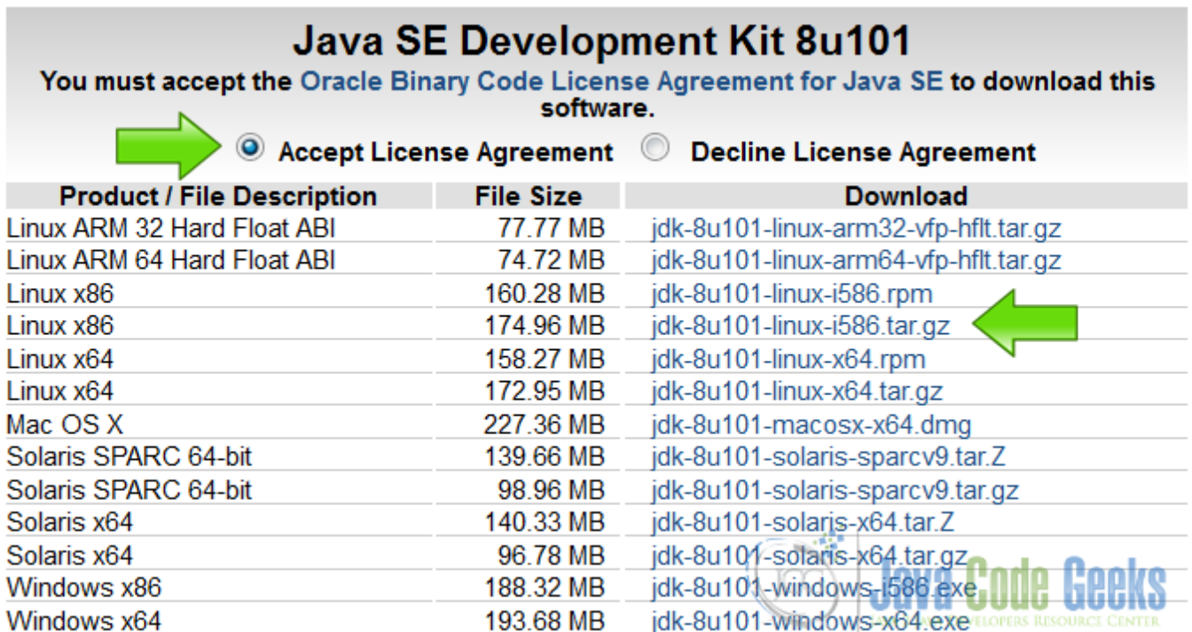
Figure 1.2: Accept agreement
