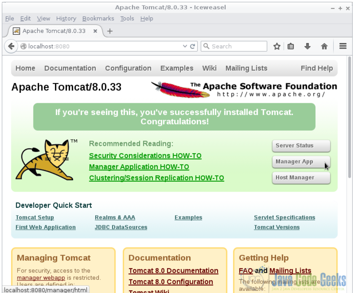
Figure 2.5: Tomcat Welcome
