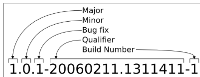
Figure 3-3: Version parsing
