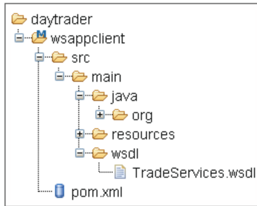
Figure 4-5: Directory structure of the wsappclient module
