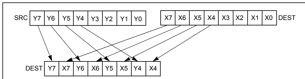
Figure 4-12. PUNPCKHBW Instruction Operation Using 64-bit Operands
