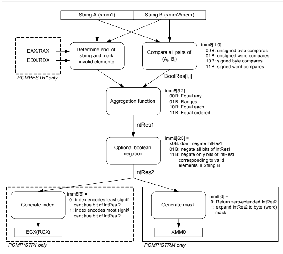
Figure 4-1. Operation of PCMPSTRx and PCPESTRx
