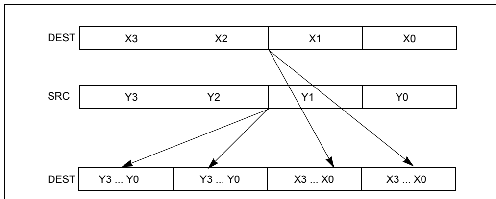
Figure 4-16. SHUFPS Shuffle Operation
