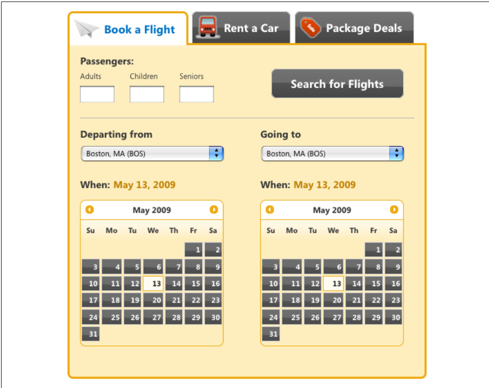
Figure 15-19. Our final design with theme classes applied to the Search button
