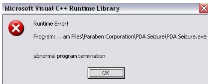
Figure 21: Runtime Error
